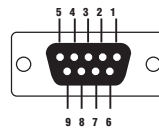
NPort® DE-311 (RS-232/422/485, DB9 female connector)
