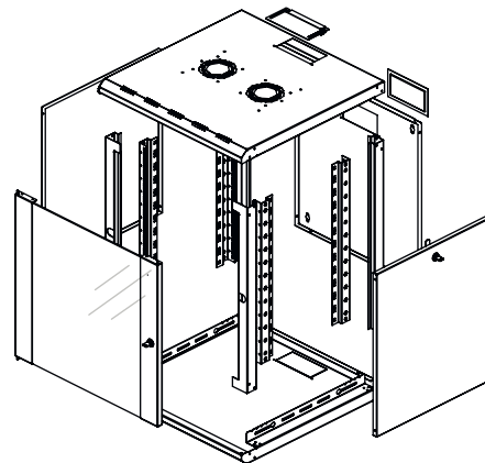
EXPLODED VIEW
