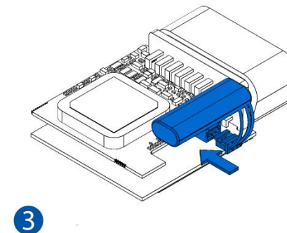
Figure 5 Battery connection
