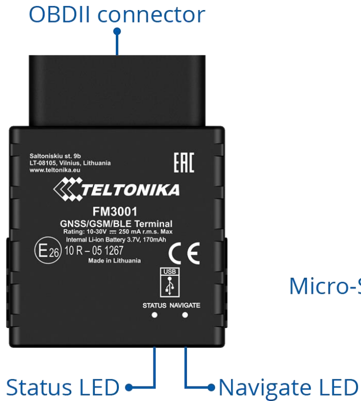
Figure 1 FM3001 device view
