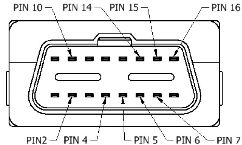
Figure 2 FM3001 OBDII socket pinout
