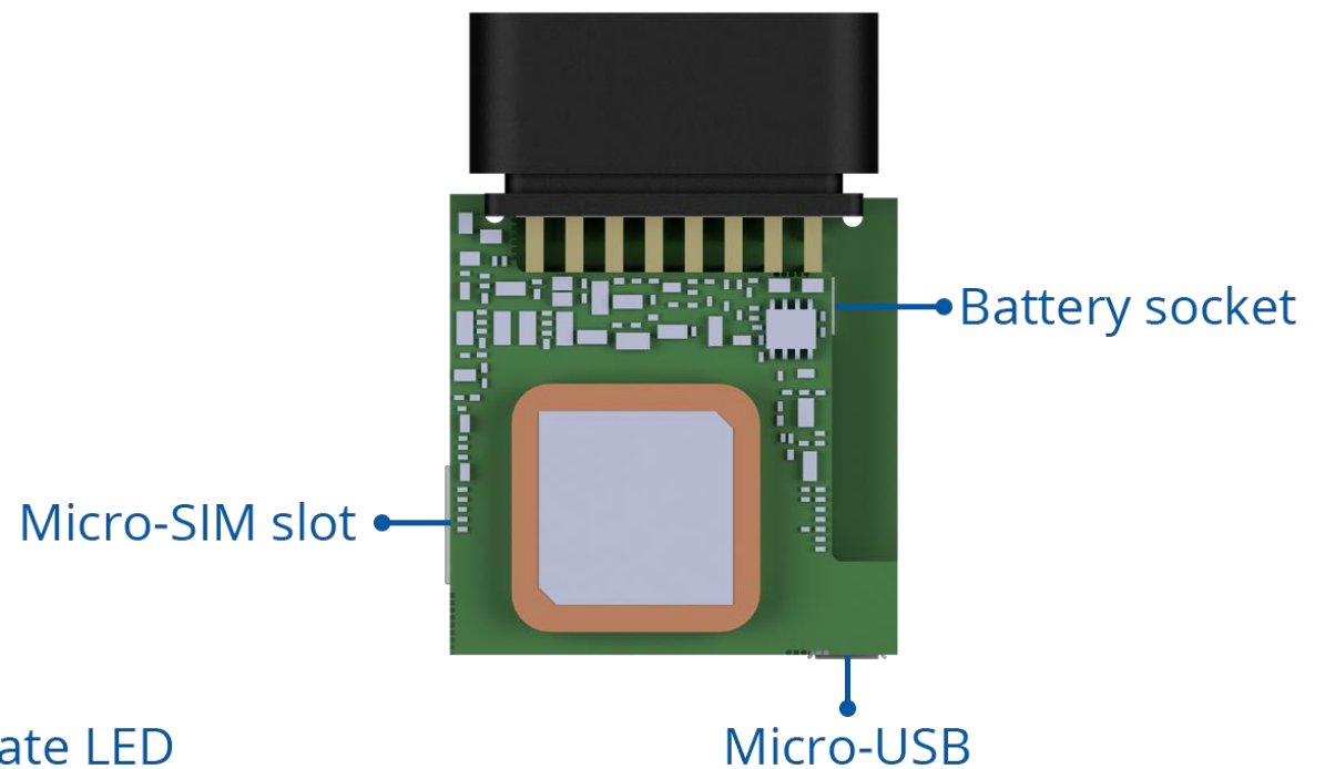
Figure 1 FM3001 device view
