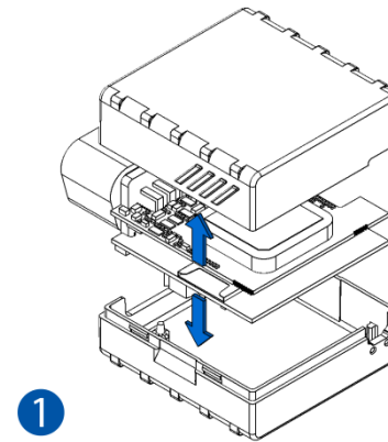
Figure 3 Cover removal
