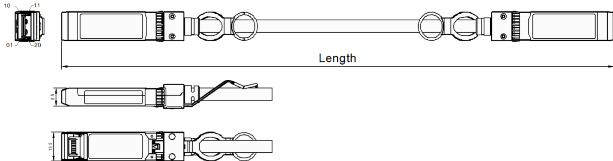
Figure 4. Mechanical Outline
