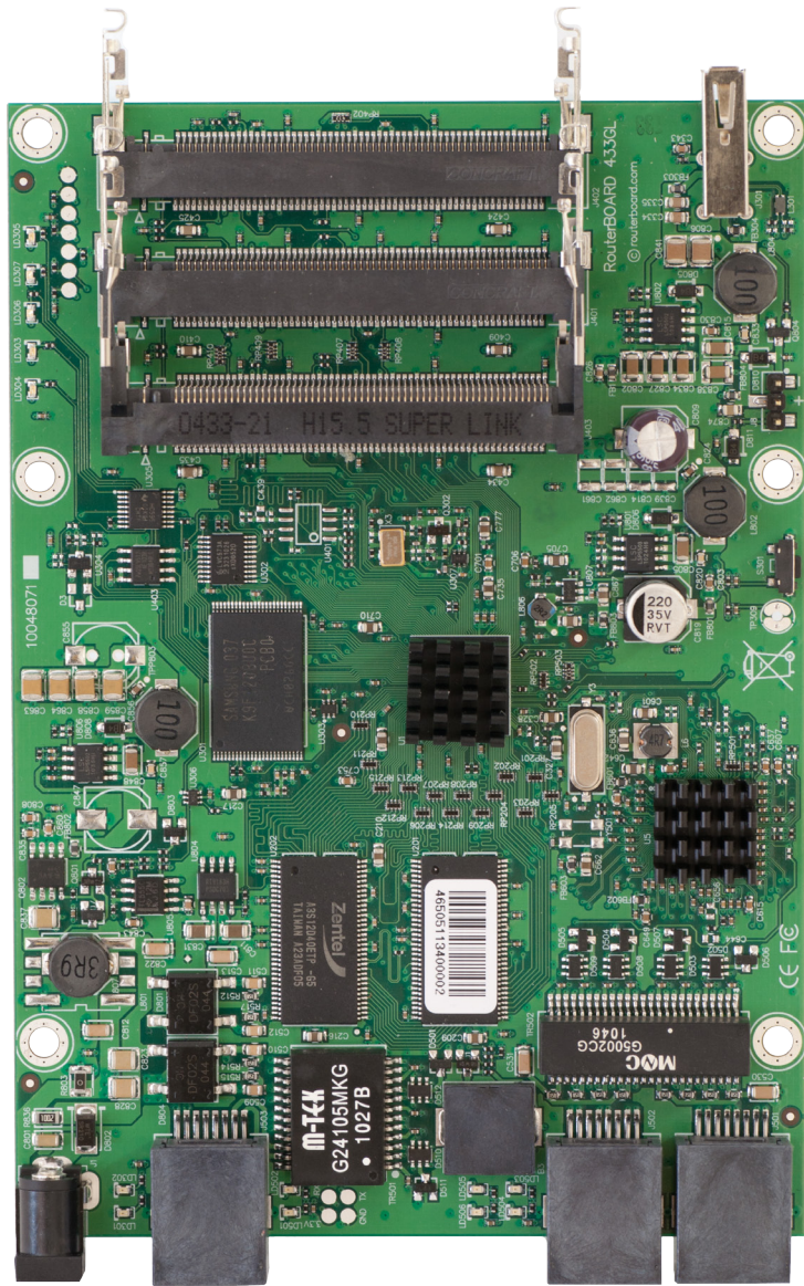
RB433GL
