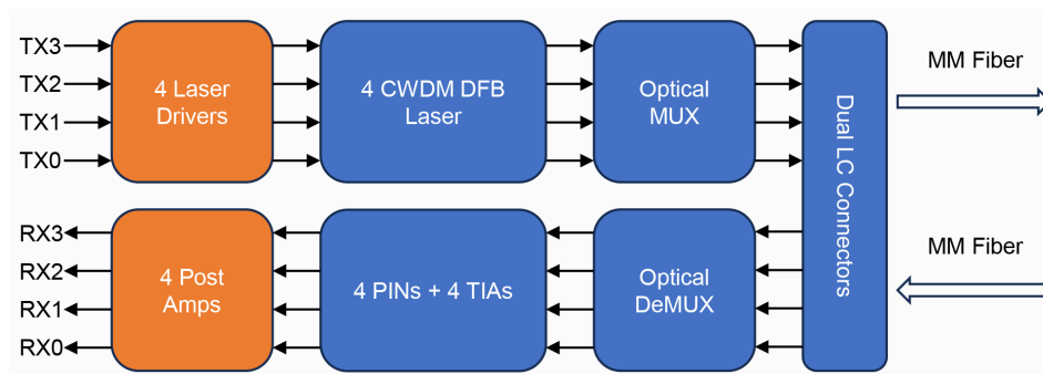
Figure 1. Transceiver Block Diagram for Applications over Multimode Fiber
