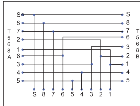
Pin Out:
