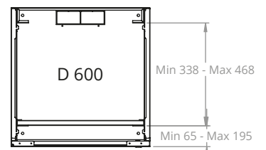
MAX/ MIN EQUIPMENT MOUNTING DISTANCE (600)
