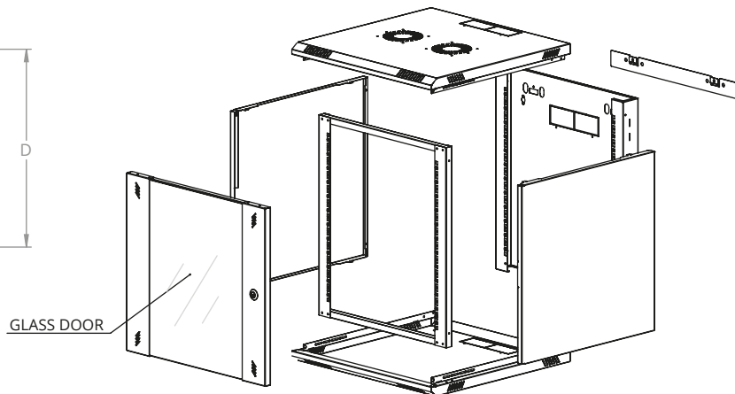
EXPLODED VIEW
