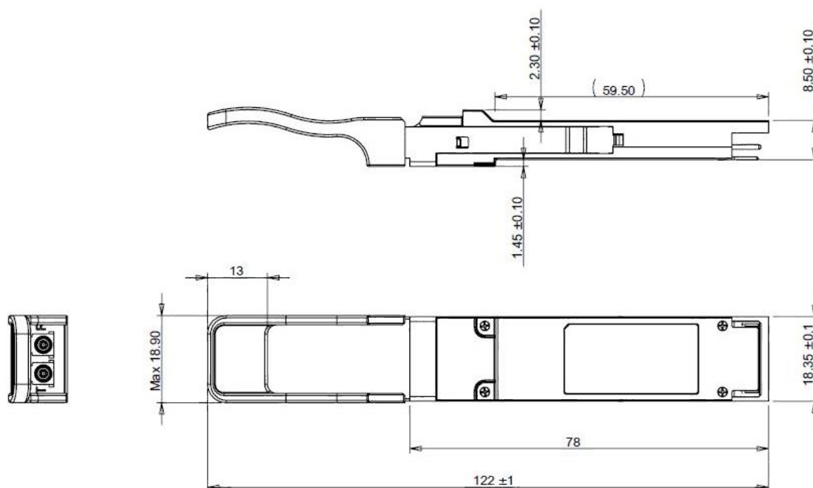
Figure 4. Mechanical Outline
