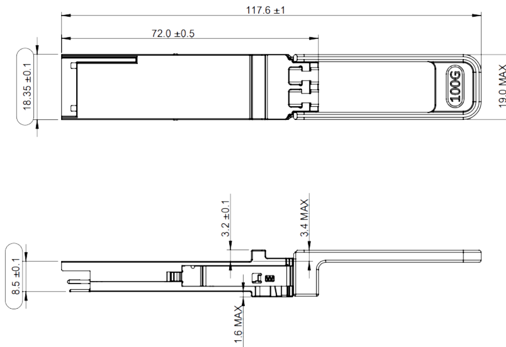
Figure 5. Mechanical Outline
