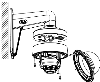
Figure 2-14 Attach the Back Box to the Mount
