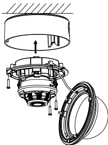
Figure 2-3 Fix the camera to the Ceiling
