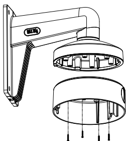
Figure 2-6 Attach the Base Plate to the Mount
