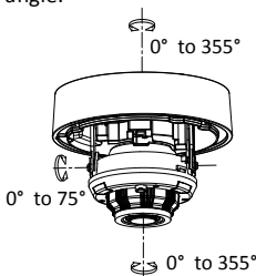
Figure 2-10 3-Axis Adjustment
