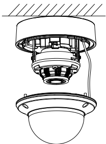
Figure 2-11 Fit the Black Liner Back
