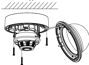
Figure 2-9 Attach the Back Box
