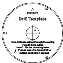
Figure 2-7 The Drill Template
